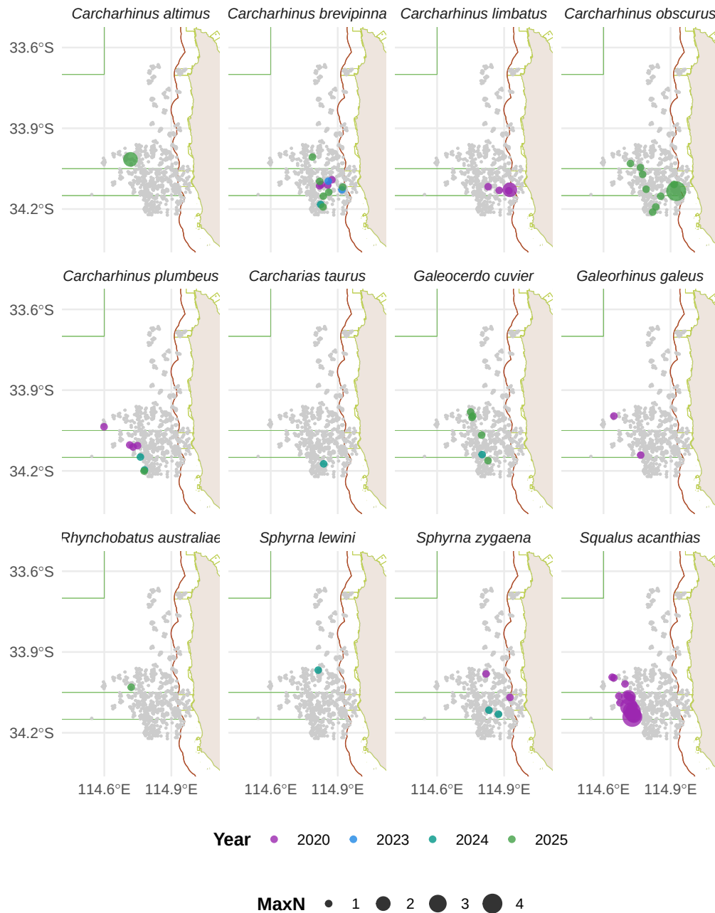
Figure A1.15.1: Occurrence of threatened sharks and rays in stereo-BRUV imagery. Points are scaled by abundance (MaxN) and coloured by survey year; grey points show every stereo-BRUV deployment, so a panel with no coloured points is a genuine absence rather than an absence of sampling. Commonwealth and state marine park boundaries are shown. The red line delimits state and commonwealth waters.
